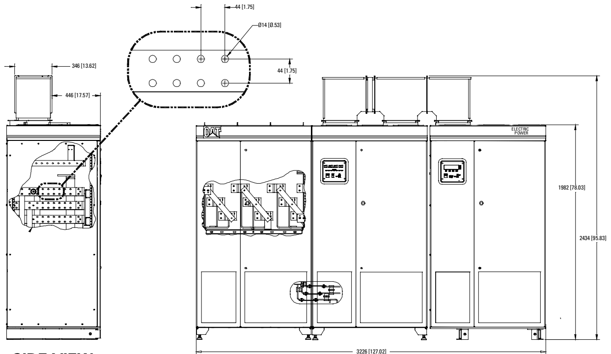
SIDE VIEW
