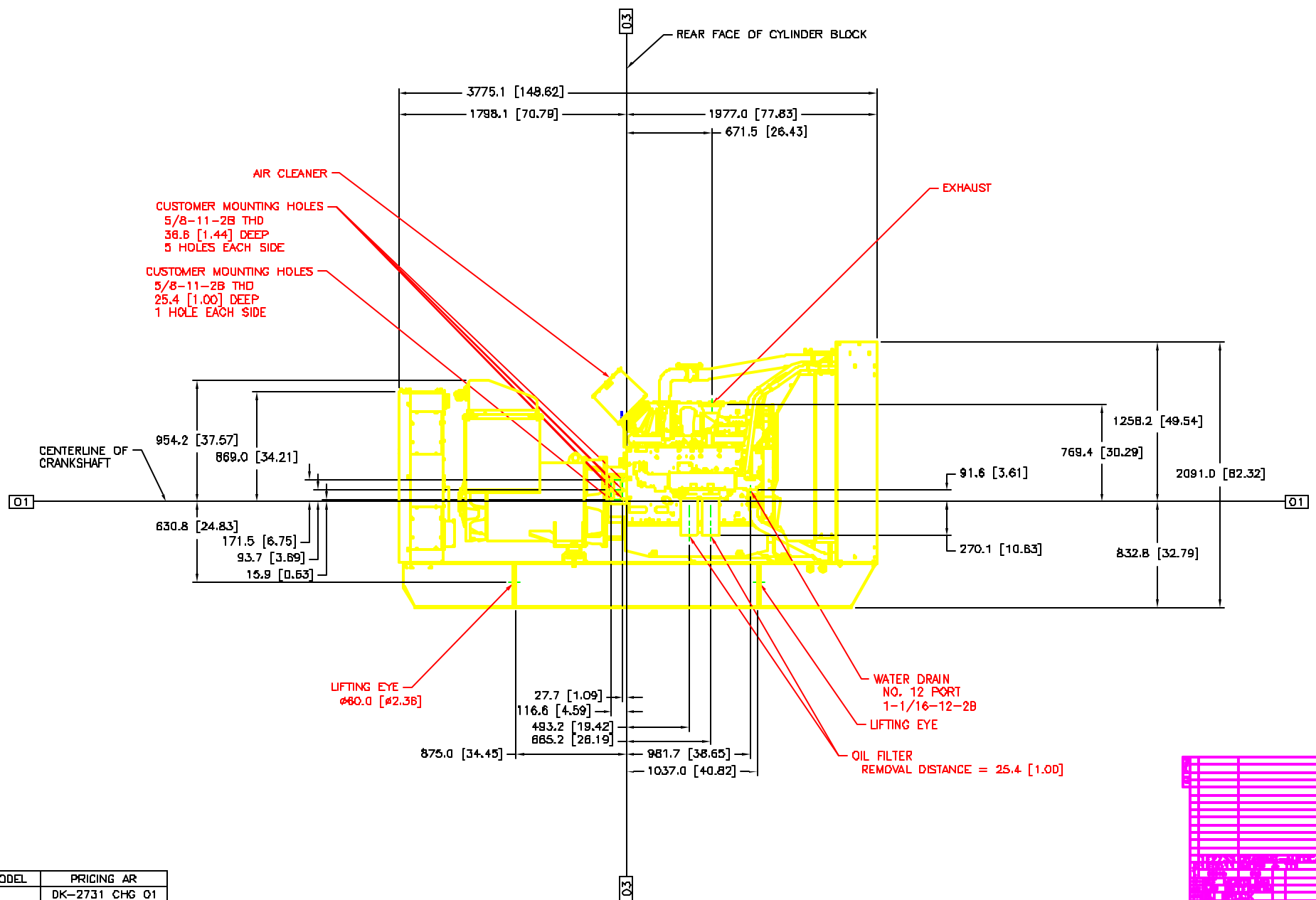
CAT C15 PACKAGE GENSET DWG# 278-1044 CHG 00 METRIC [INCH] RIGHT SIDE VIEW DK-2731 CHG 01 SHOWN
